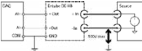
The schematic on the figure above shows how to connect the Entube-DE-HB between the high voltage signal source and the digitizer.
